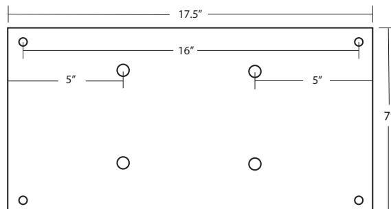
Wall Mount Bracket - double (sold separately; part number: EVCS-UCR-WMB-DBL)
