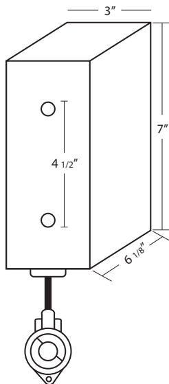
Universal Cable Retractor (part number: EVCS-UCR)
