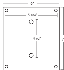
Wall Mount Bracket - single (sold separately; part number: EVCS-UCR-WMB-SGL)
