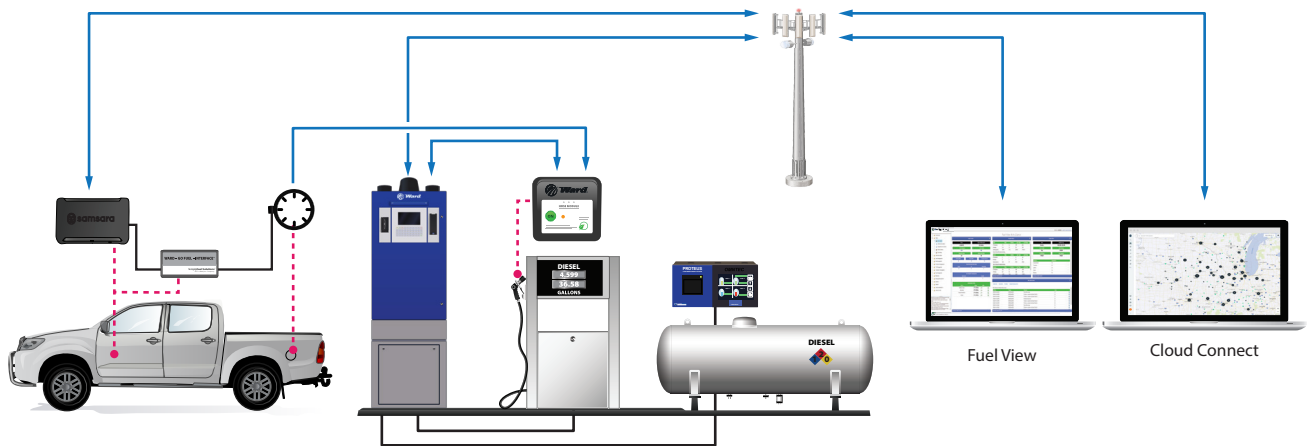
Sample Ward Fuel Management System using a Samsara Gateway. Sites and configurations will vary.
